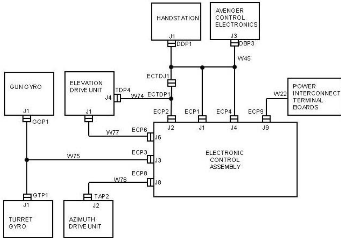
FIGURE 53. Example of a cable interconnect diagram.
