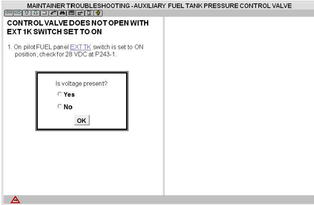
FIGURE A-6. Example of a troubleshooting procedure - Continued (Sheet 2 of 5)
