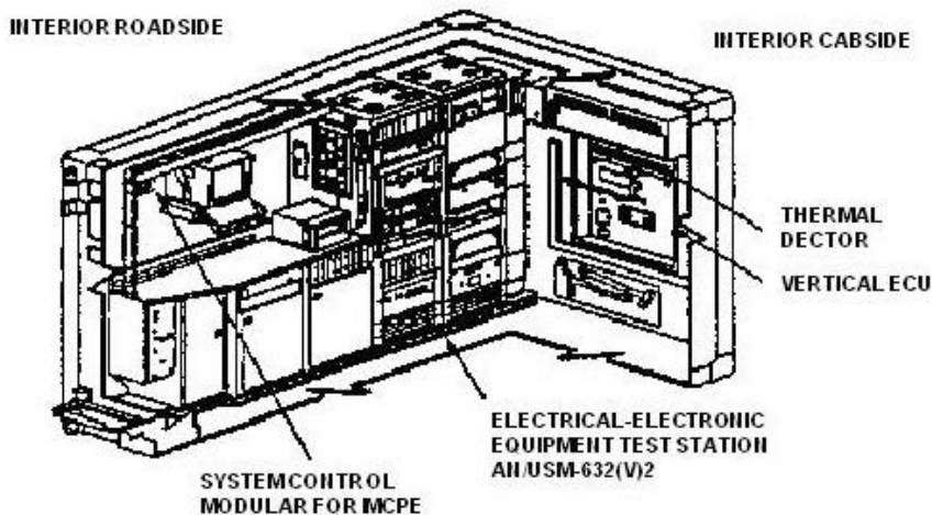
Figure 2. Interior Components
