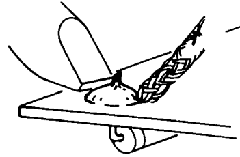
FIGURE D-47. Desoldering with a Braided Wick.
